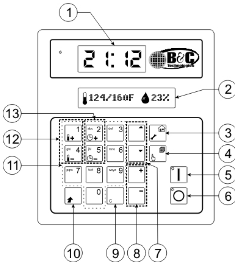
Figure 2.1: M720 Display and Keypad Detail
