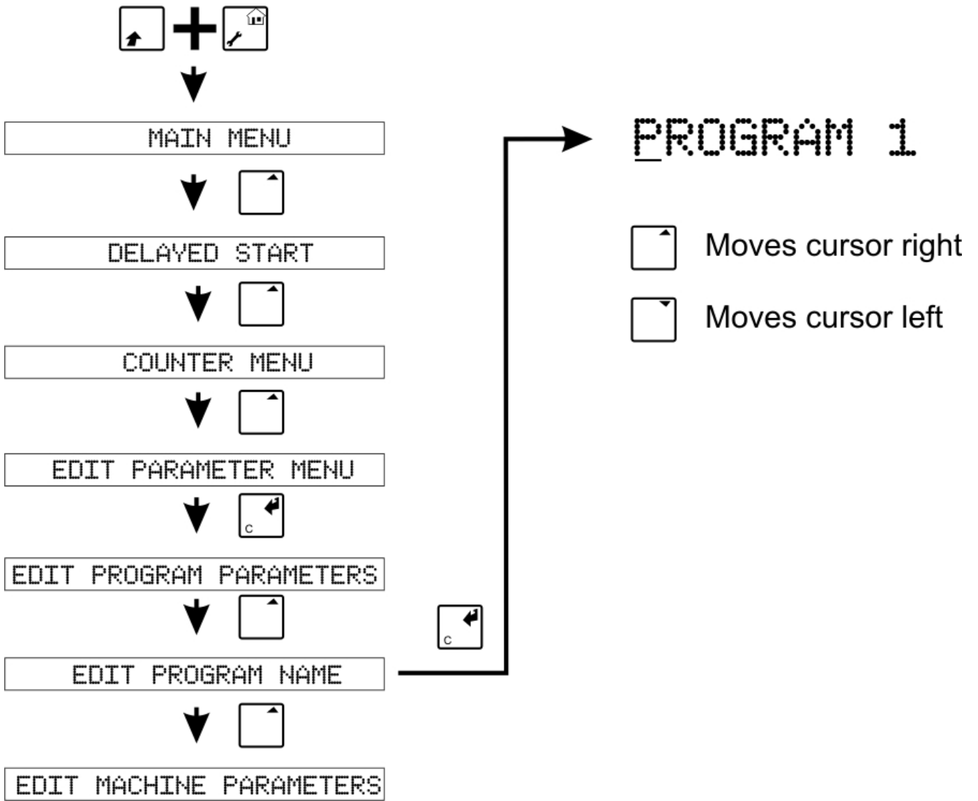
Figure 4.3: M720 Program Naming Menu
