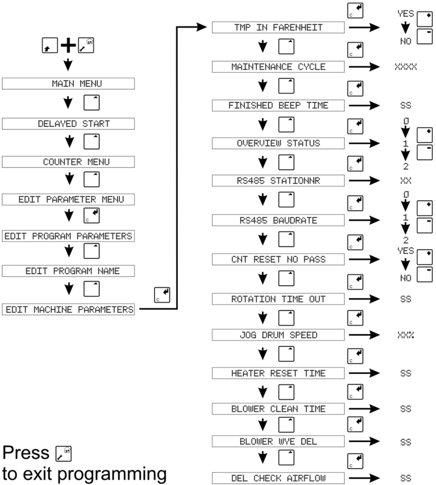
Figure 4.4: M720 Machine Parameter Menu
