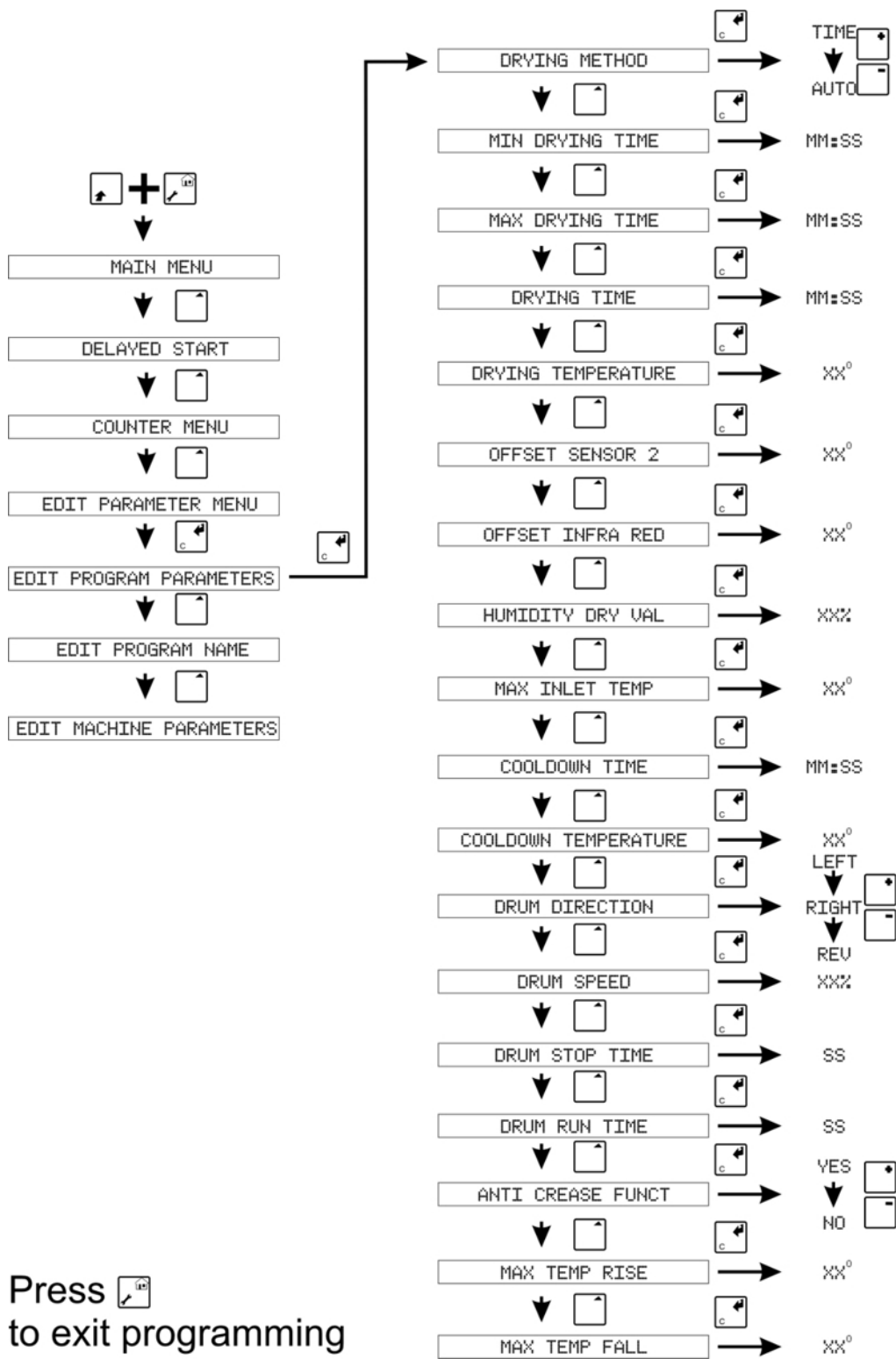
Figure 4.2: M720 Program Parameter Menu
