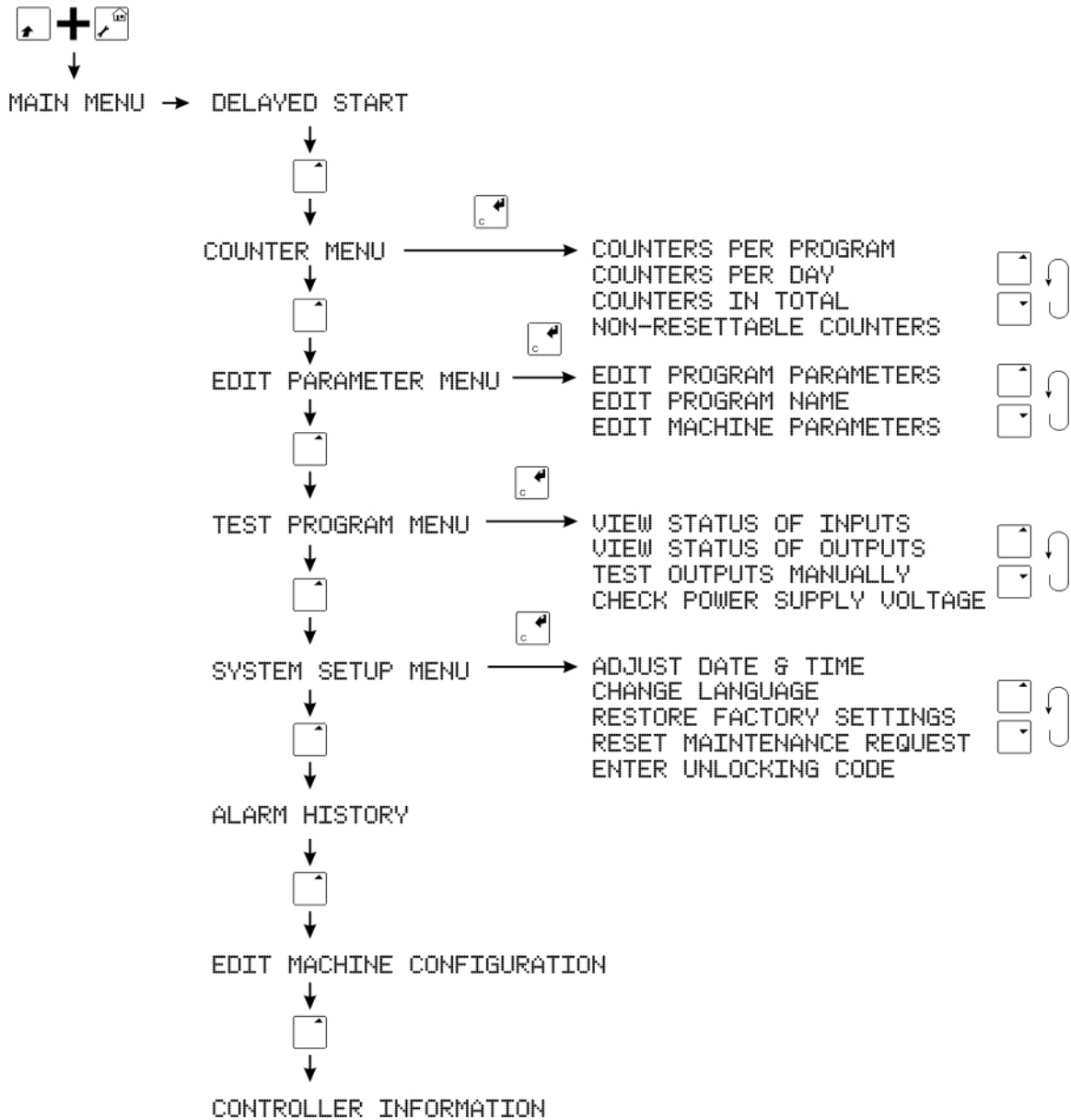
Figure 4.1: M720 Menu Structure
